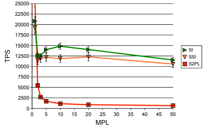
(a) Relative throughput of SI, S2PL and Serializable SI without log flushes
