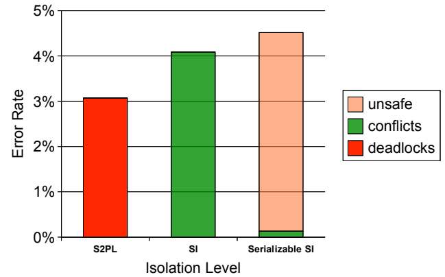
(b) Relative error rates of SI, S2PL and Serializable SI at MPL 20 without log flushes
